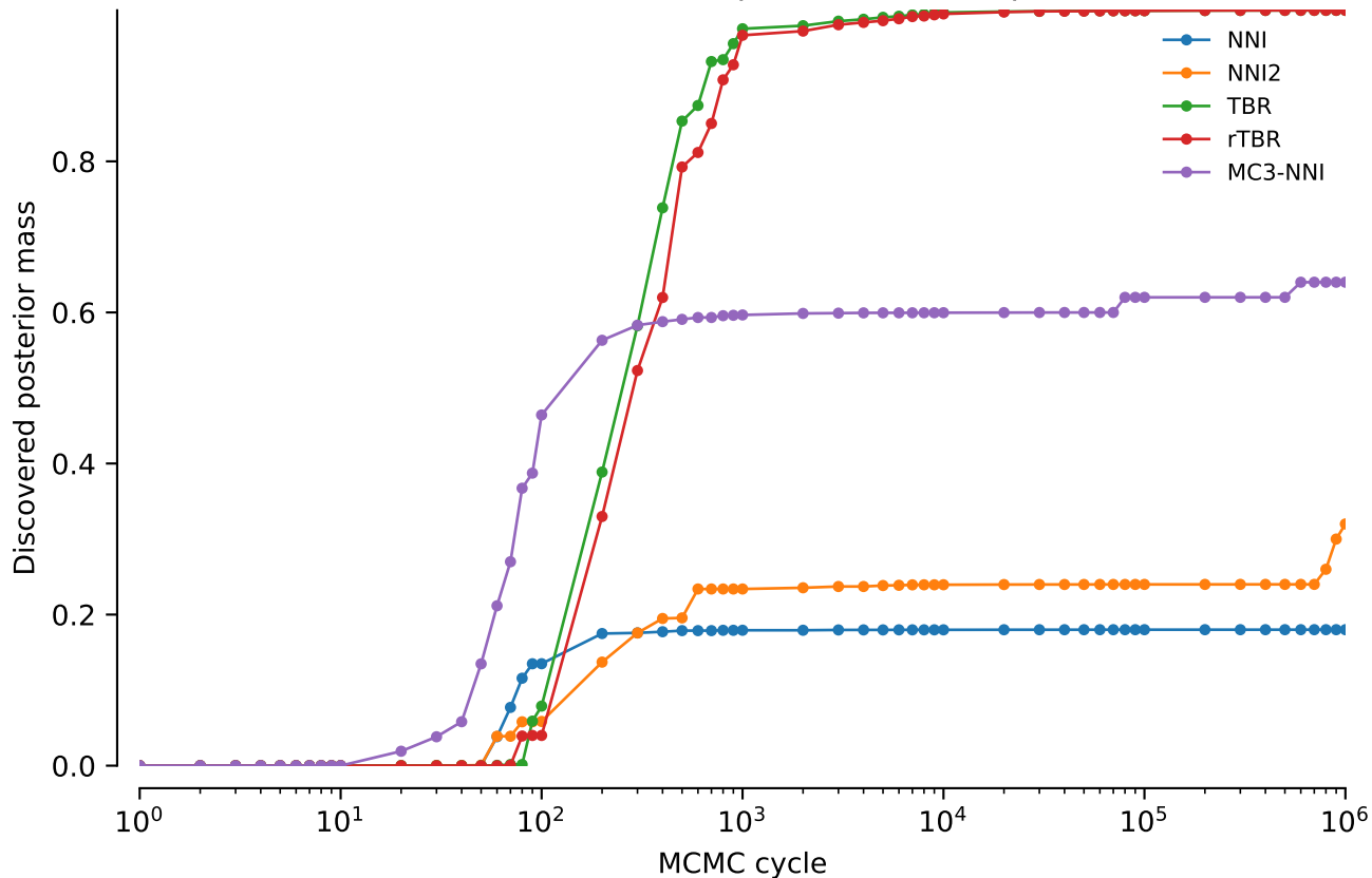
vert.nd6.tw5: Discovered posterior mass: power = 0
