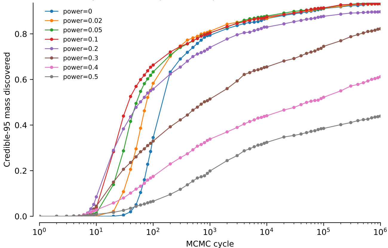
Combined alignments: NNI power comparison: Credible-95 mass discovered
