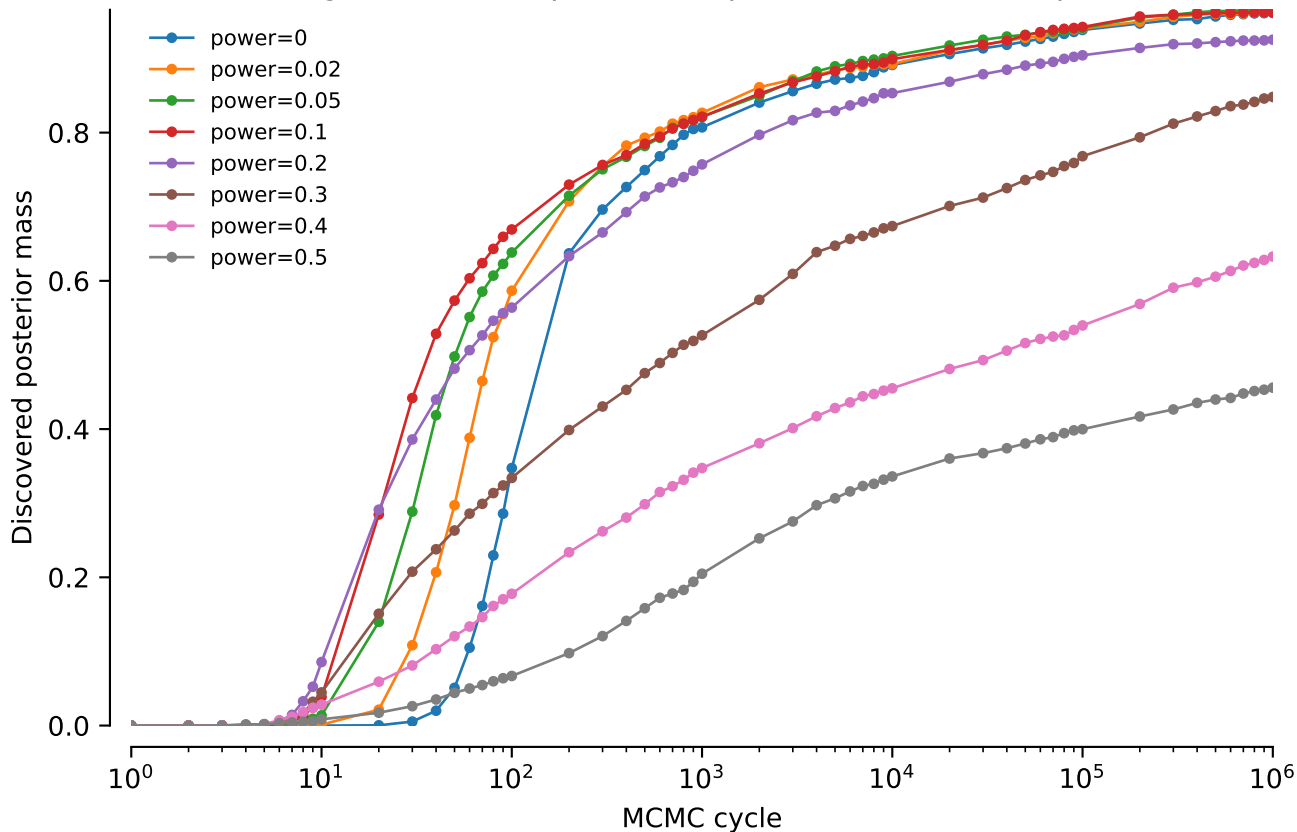
Combined alignments: NNI power comparison: Discovered posterior mass
