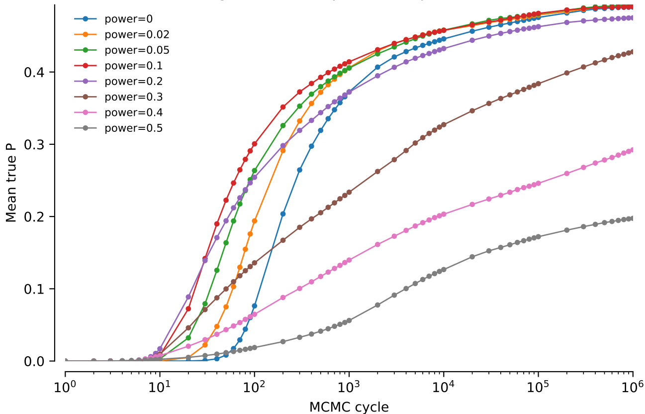
Combined alignments: NNI power comparison: Mean true P
