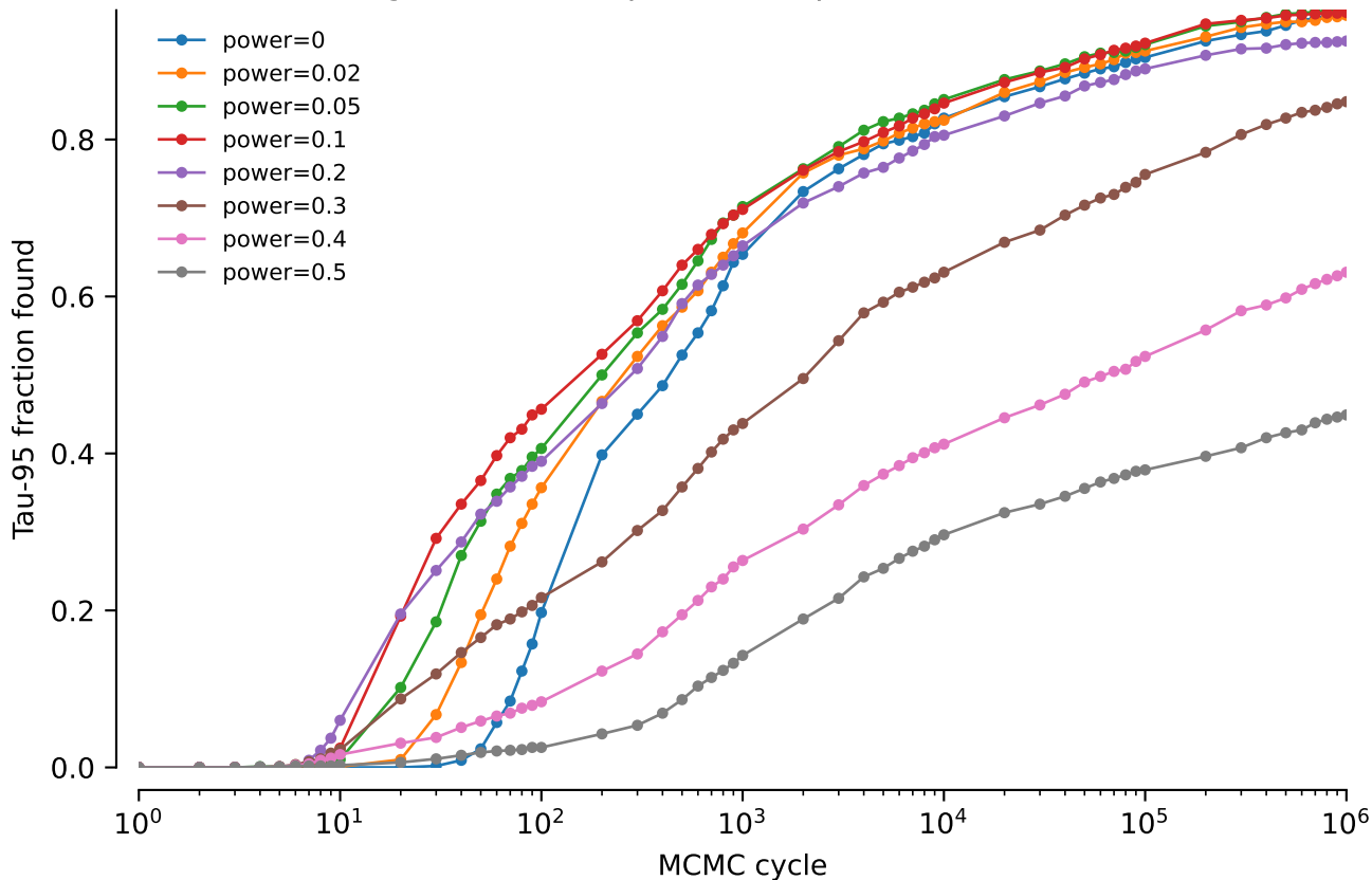
Combined alignments: NNI power comparison: Tau-95 fraction found
