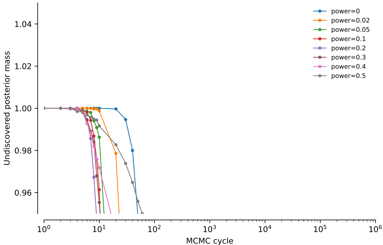
Combined alignments: NNI power comparison: Undiscovered posterior mass
