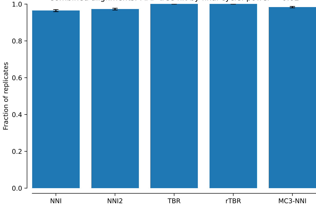
Combined alignments: MAP tree hit by final cycle: power = 0.02
