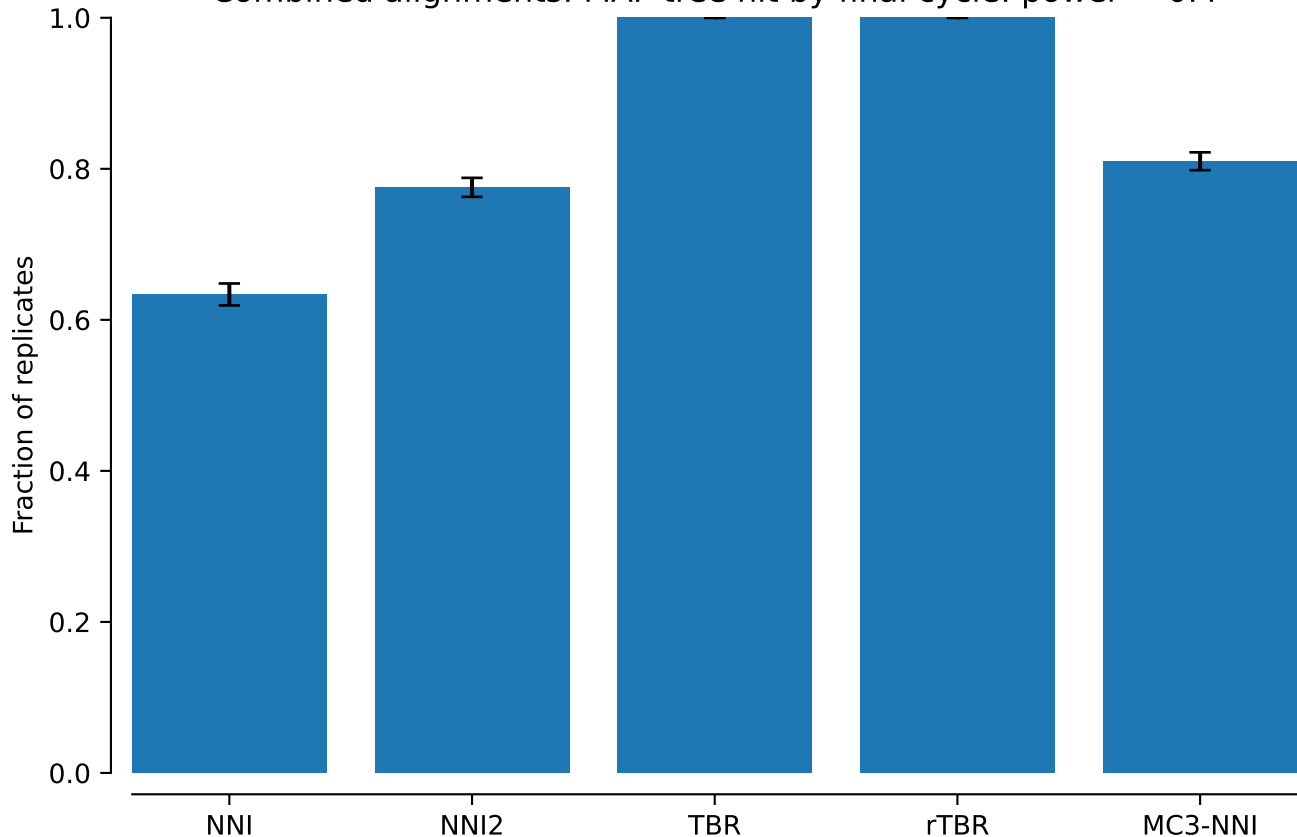
Combined alignments: MAP tree hit by final cycle: power = 0.4
