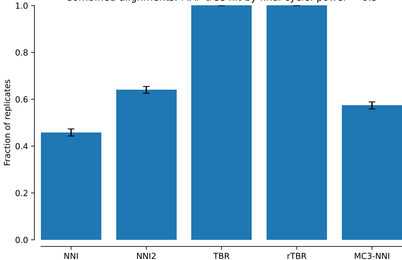
Combined alignments: MAP tree hit by final cycle: power = 0.5
