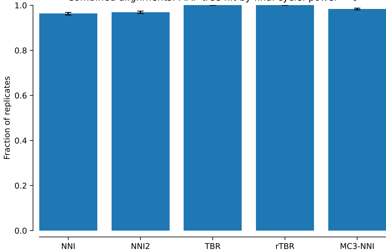
Combined alignments: MAP tree hit by final cycle: power = 0
