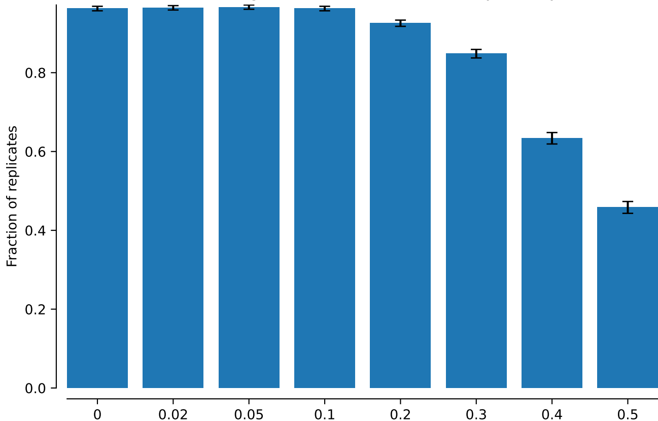
Combined alignments: NNI: MAP tree hit by final cycle
