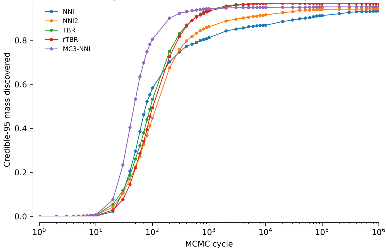
Combined alignments: Credible-95 mass discovered: power = 0.02
