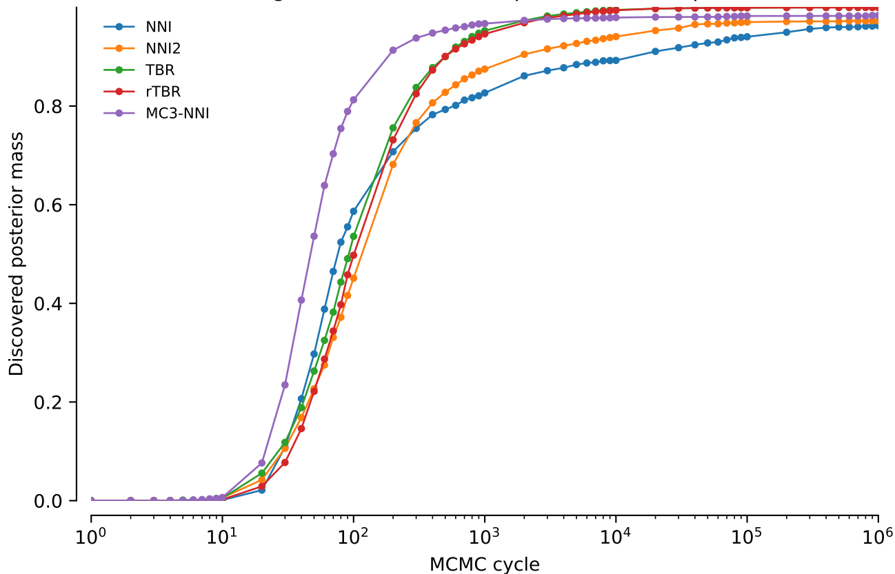
Combined alignments: Discovered posterior mass: power = 0.02
