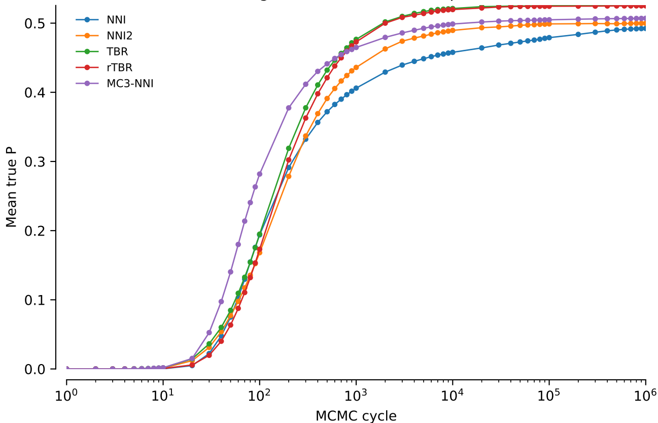
Combined alignments: Mean true P: power = 0.02
