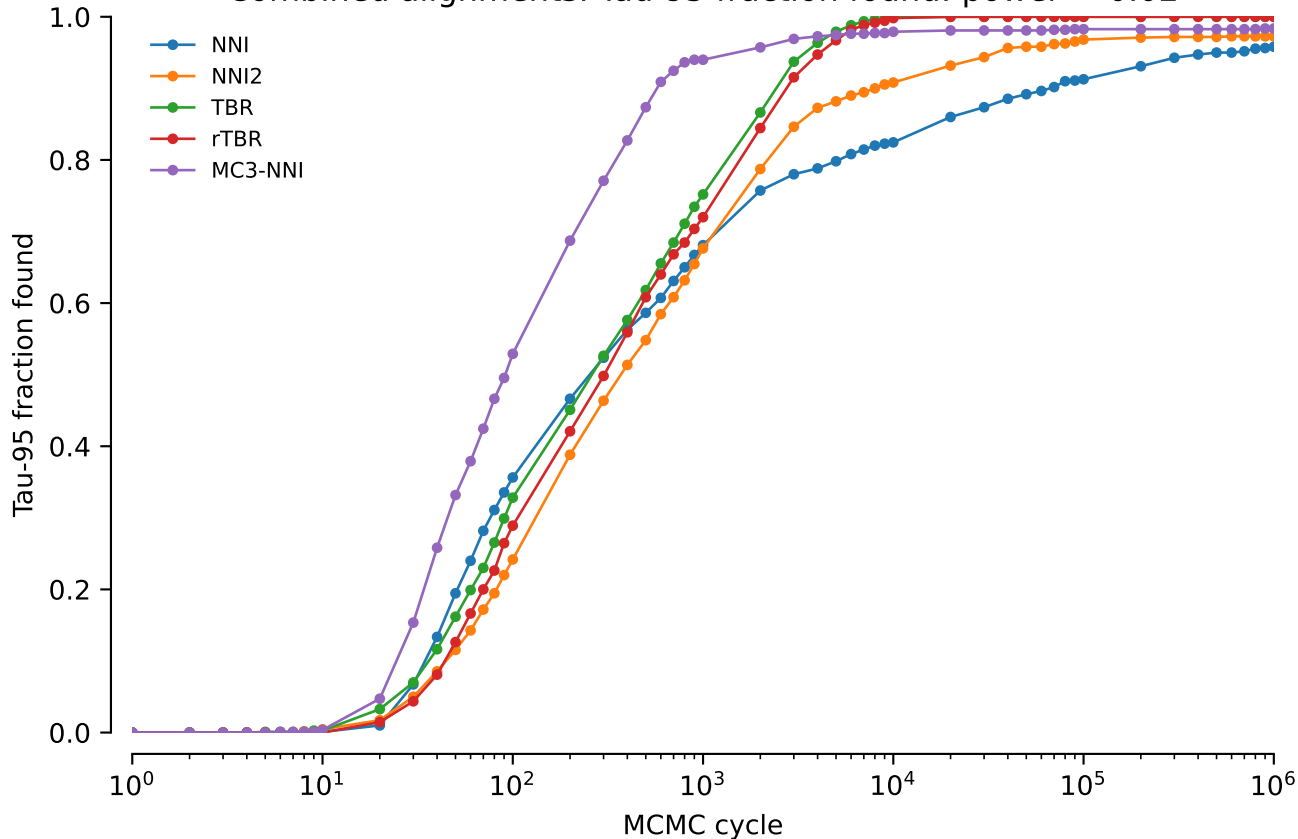
Combined alignments: Tau-95 fraction found: power = 0.02
