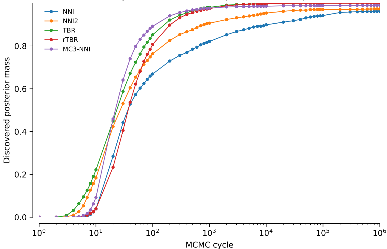
Combined alignments: Discovered posterior mass: power = 0.1
