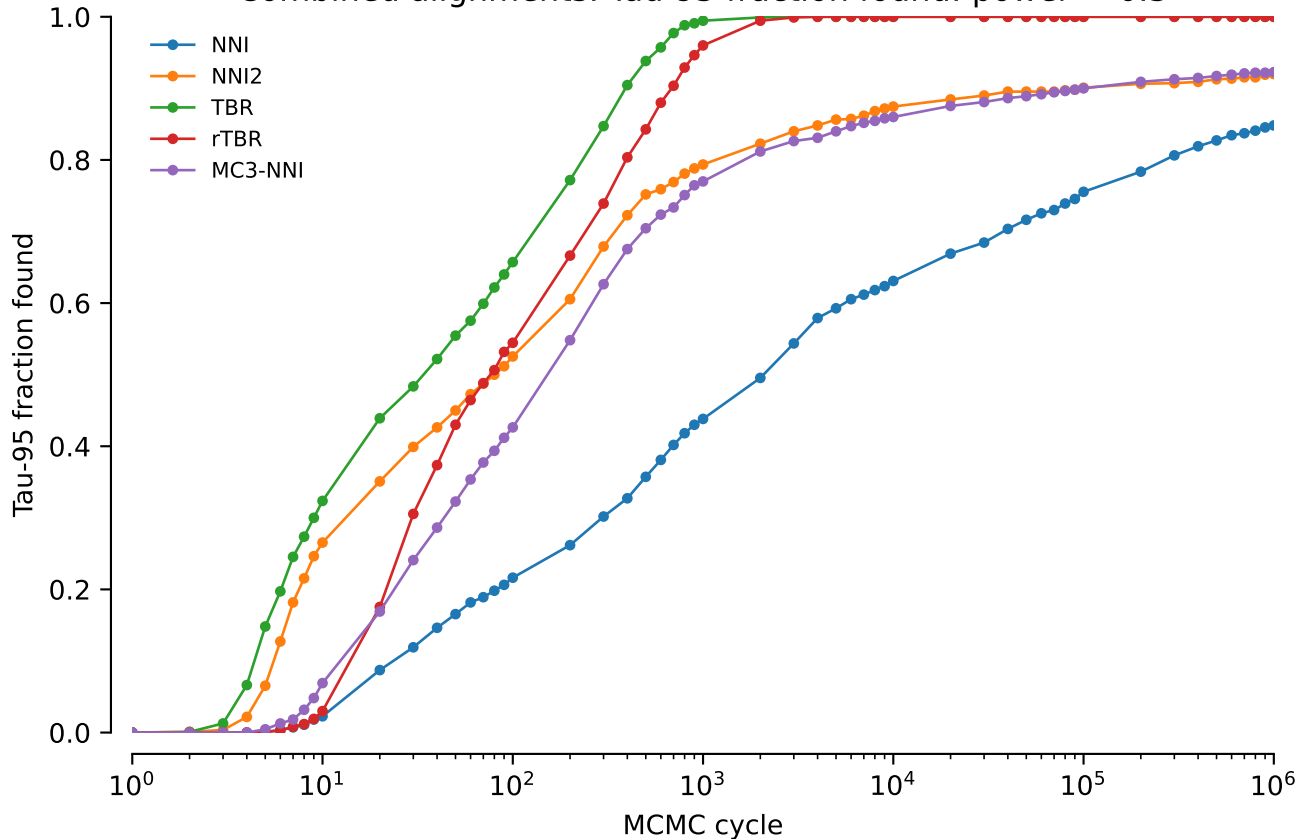
Combined alignments: Tau-95 fraction found: power = 0.3
