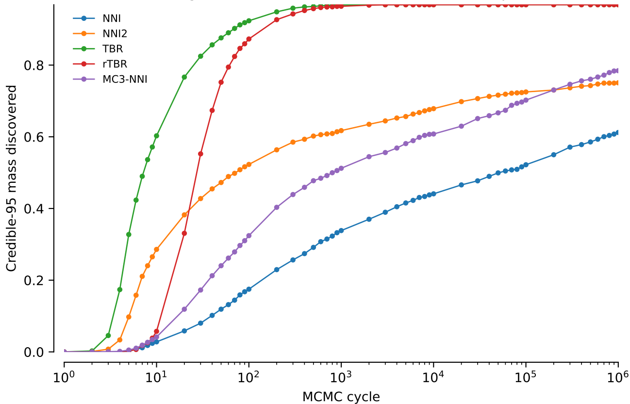
Combined alignments: Credible-95 mass discovered: power = 0.4
