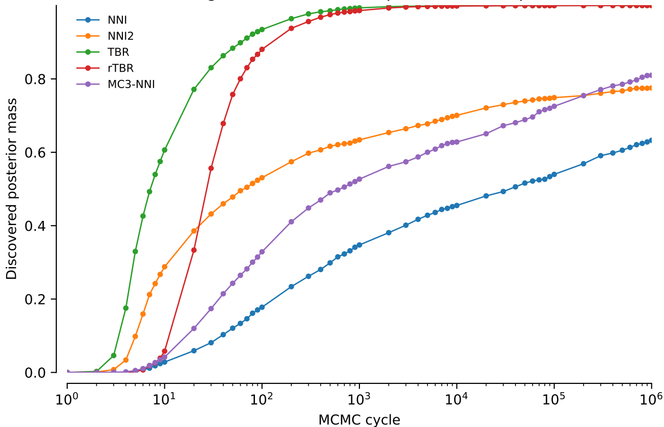
Combined alignments: Discovered posterior mass: power = 0.4
