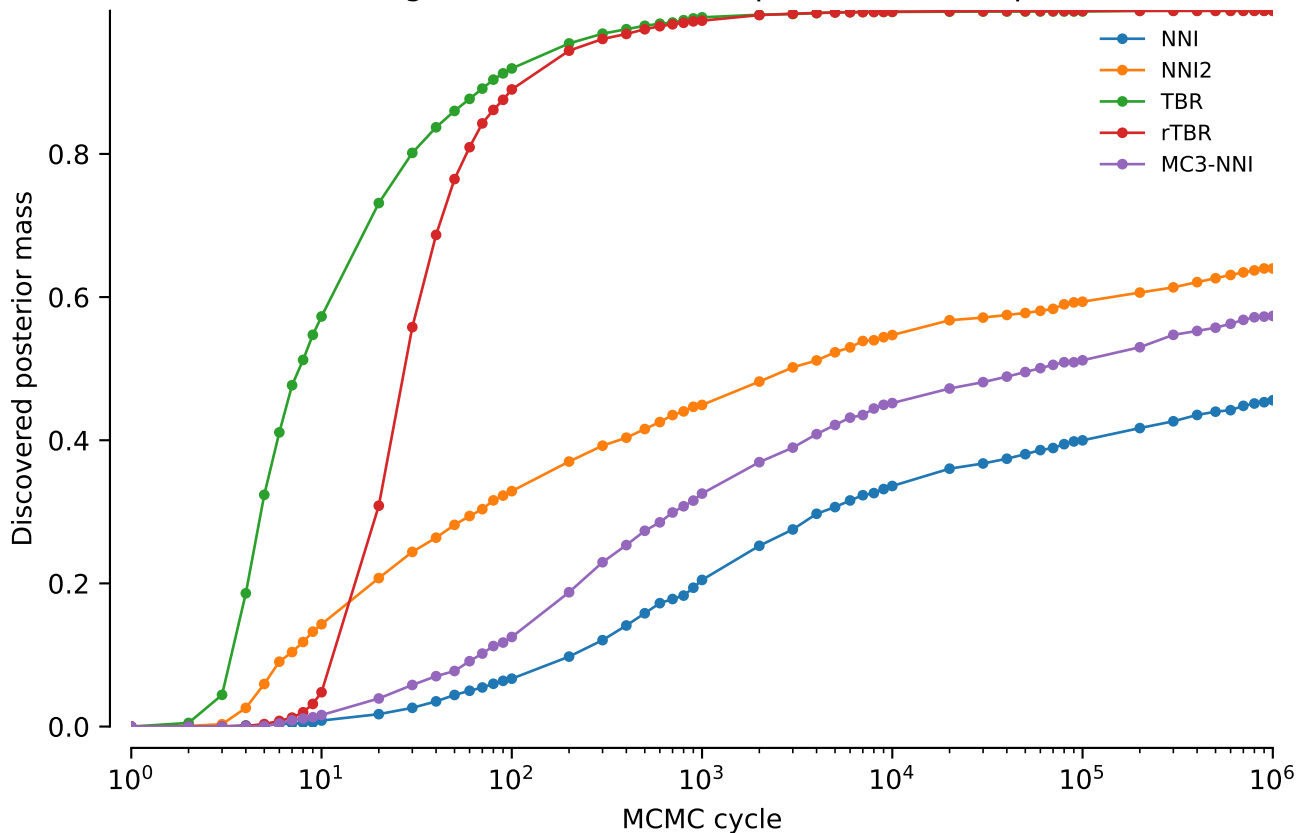
Combined alignments: Discovered posterior mass: power = 0.5
