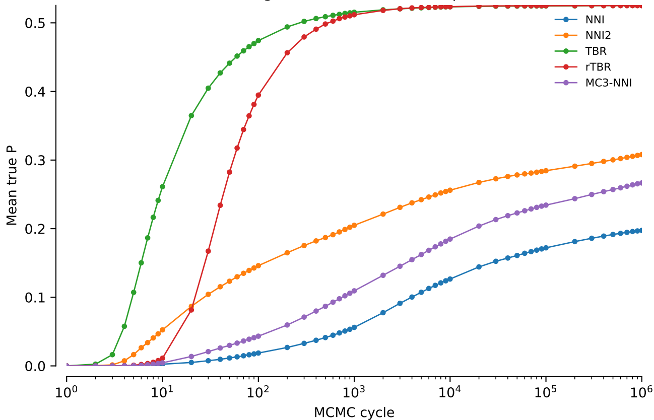
Combined alignments: Mean true P: power = 0.5
