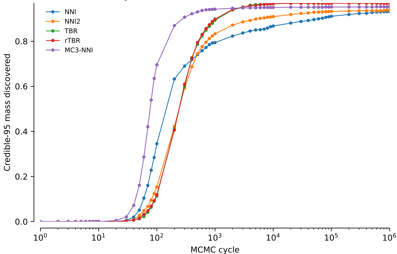
Combined alignments: Credible-95 mass discovered: power = 0
