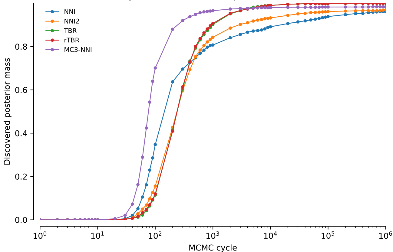
Combined alignments: Discovered posterior mass: power = 0
