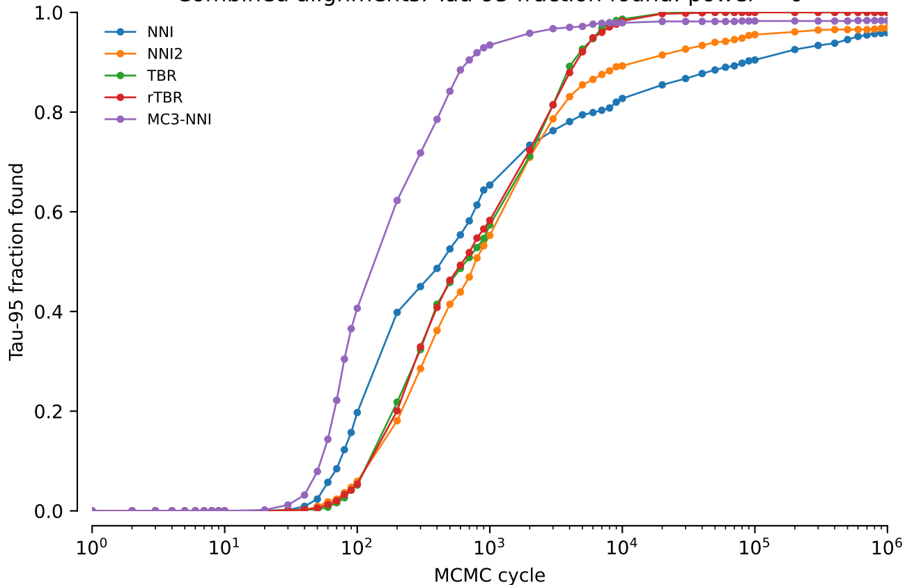
Combined alignments: Tau-95 fraction found: power = 0
