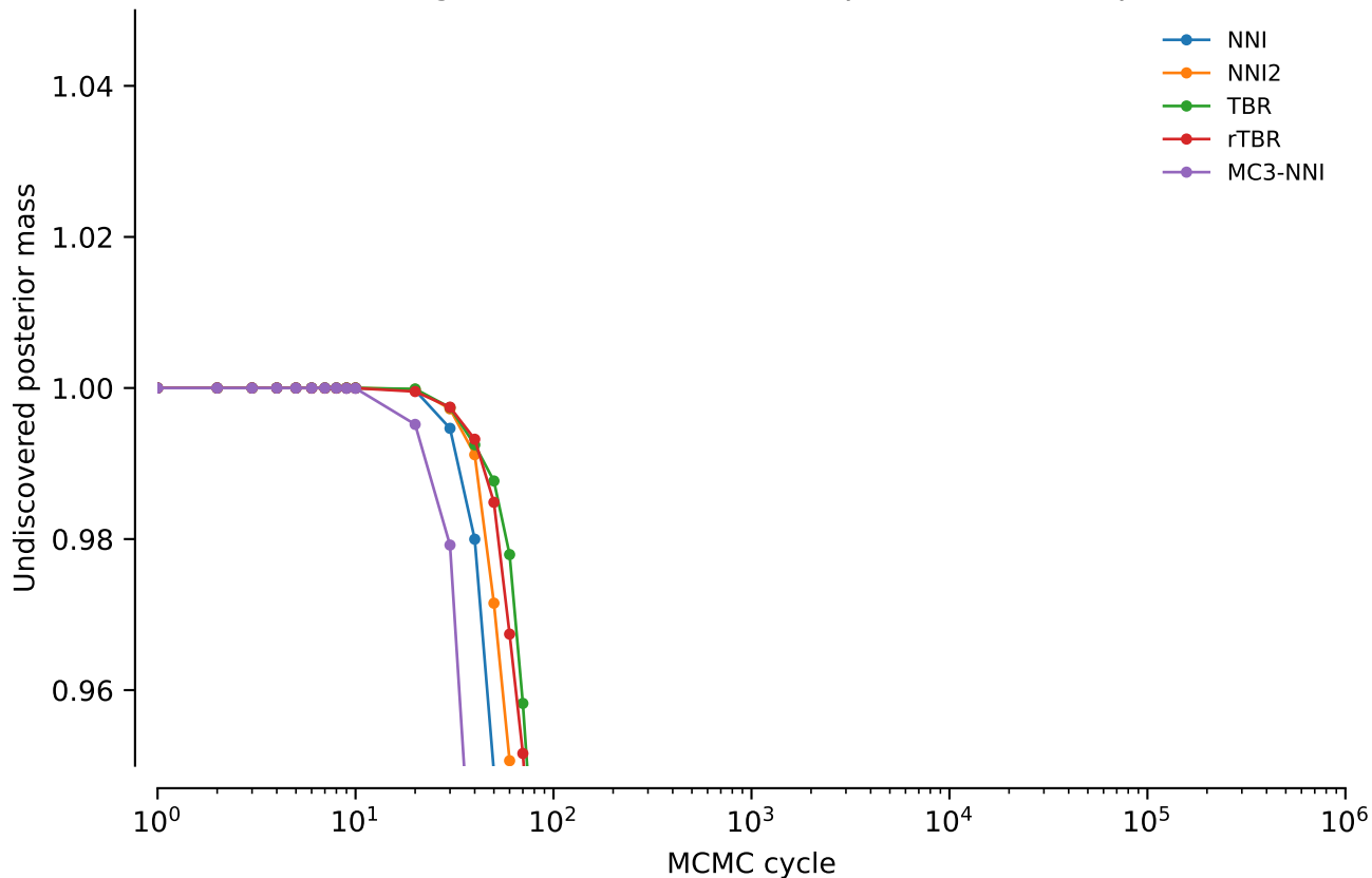
Combined alignments: Undiscovered posterior mass: power = 0
