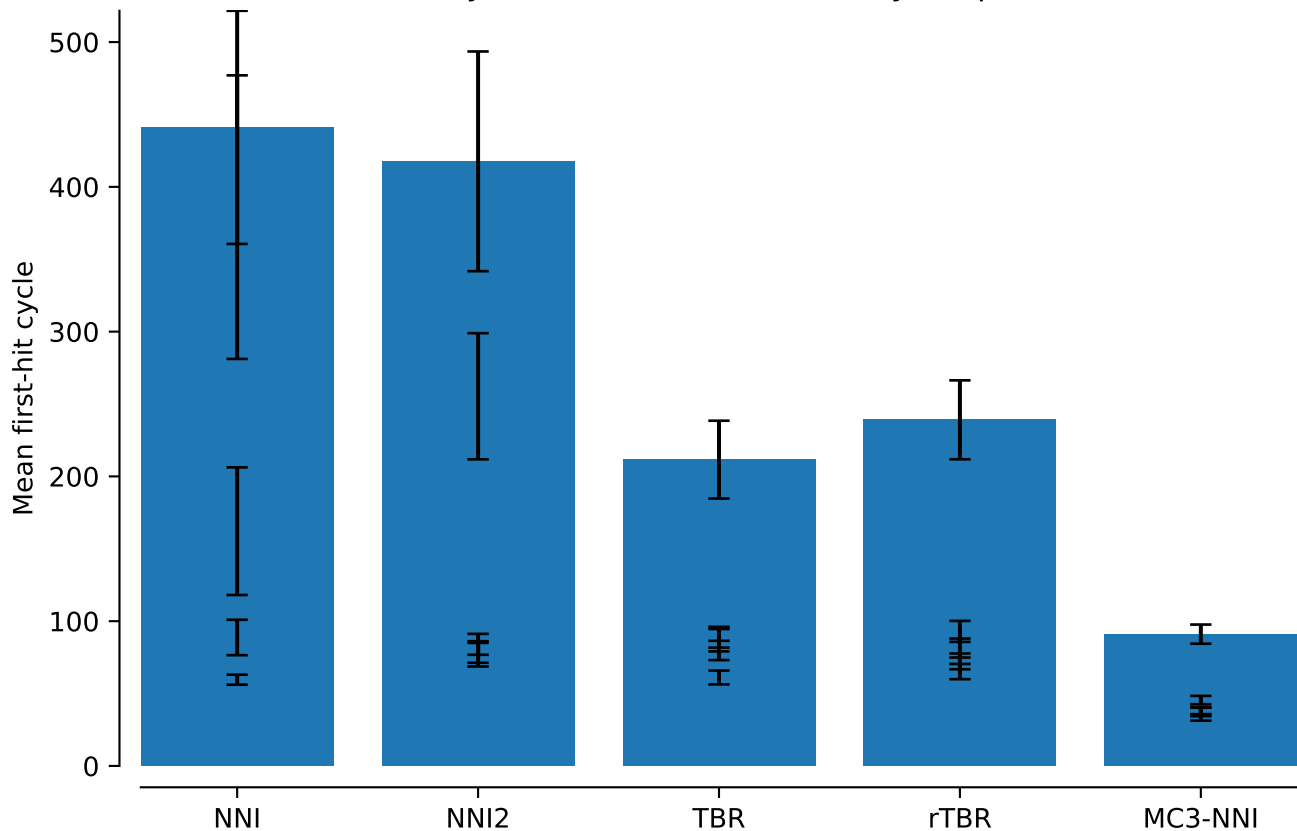
MAP first-hit cycle, non-hits set to max cycle: power = 0.02
