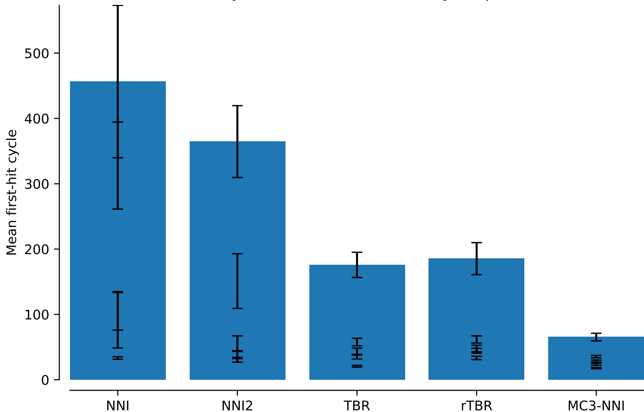
MAP first-hit cycle, non-hits set to max cycle: power = 0.05
