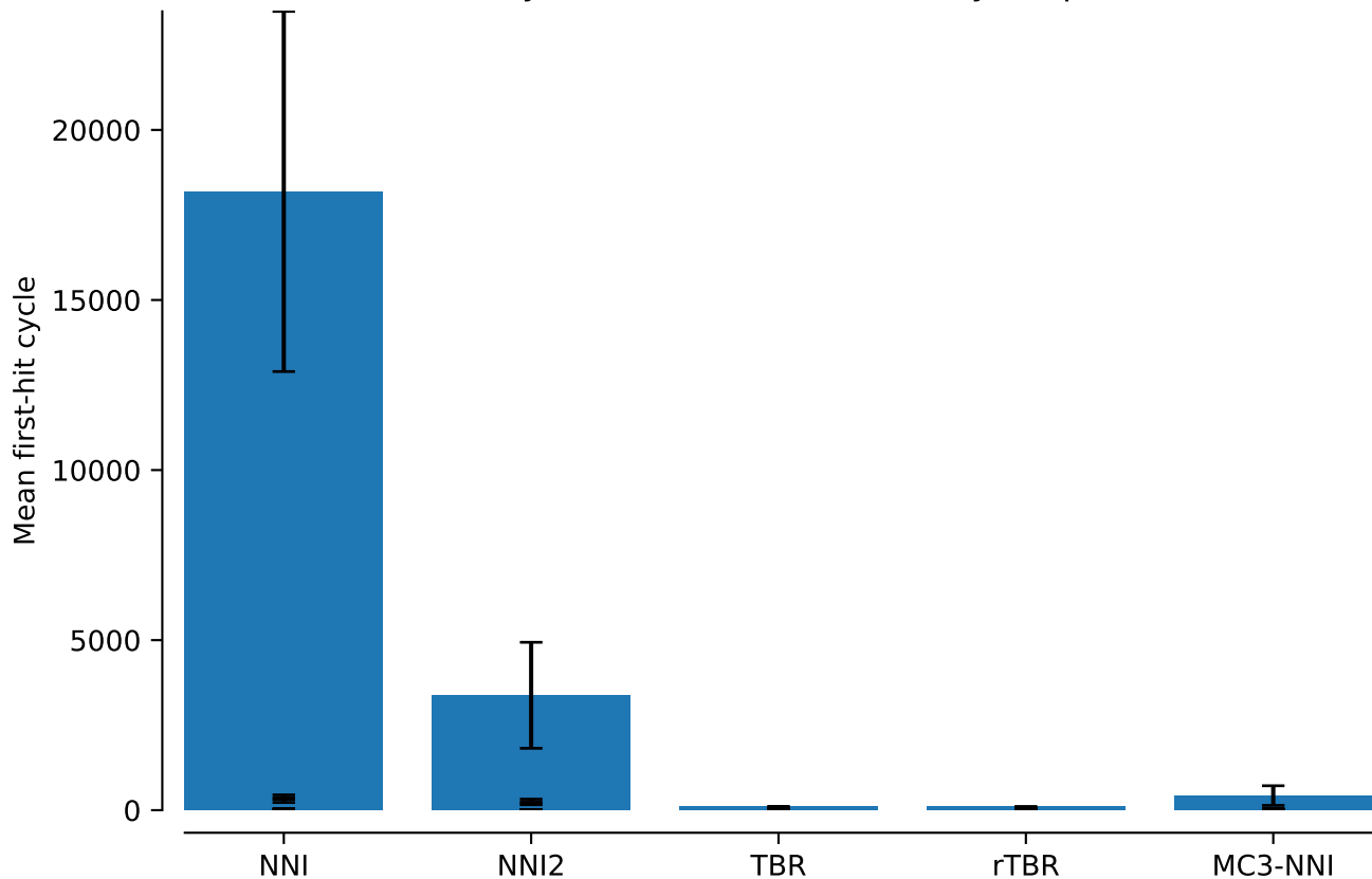
MAP first-hit cycle, non-hits set to max cycle: power = 0.1
