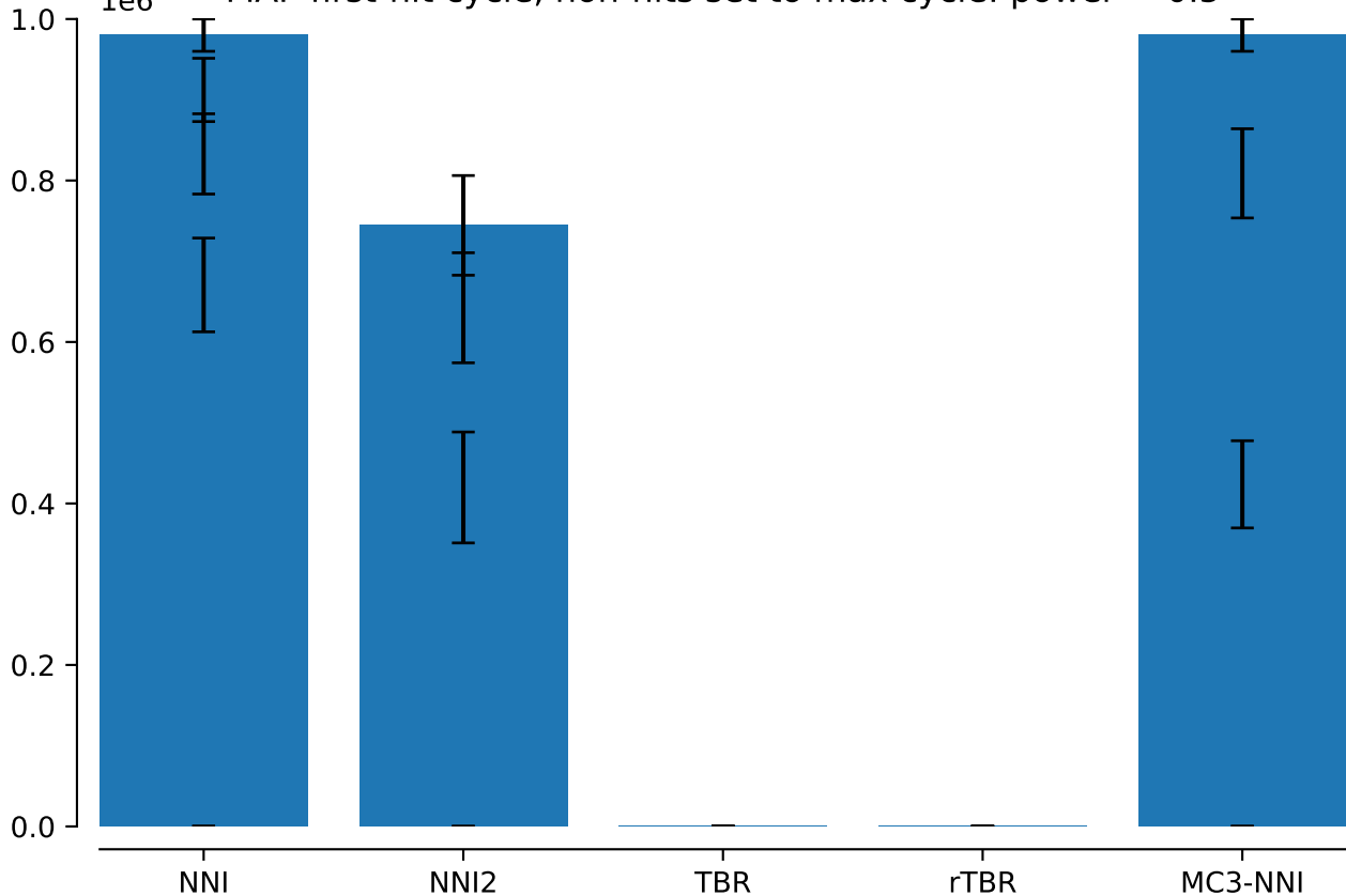
MAP first-hit cycle, non-hits set to max cycle: power = 0.5
