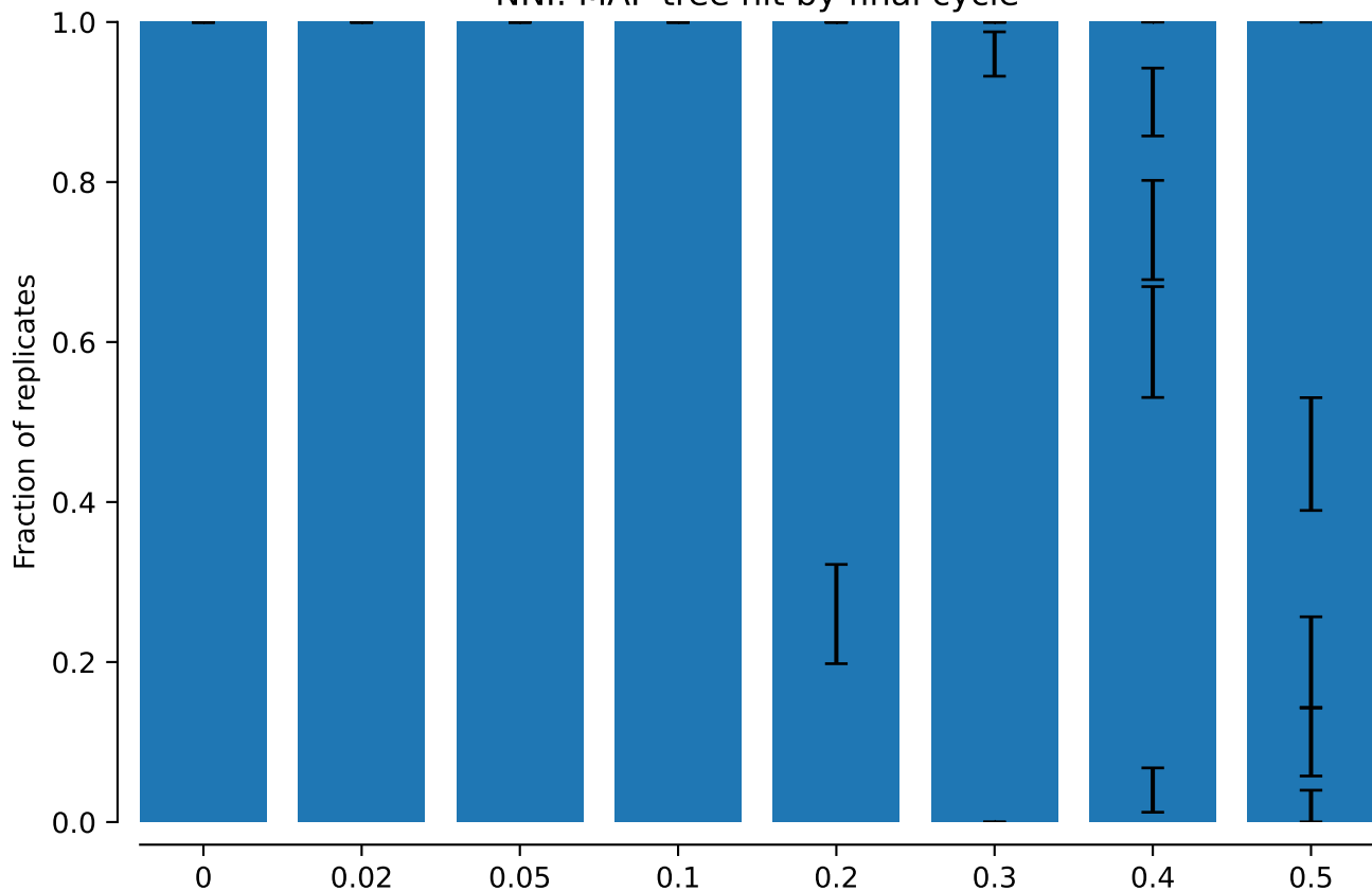
NNI: MAP tree hit by final cycle
