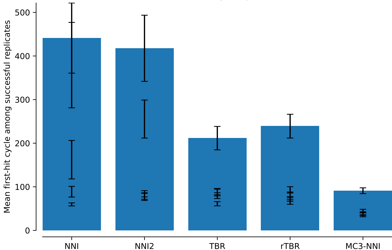
Mean MAP first-hit cycle: power = 0.02
