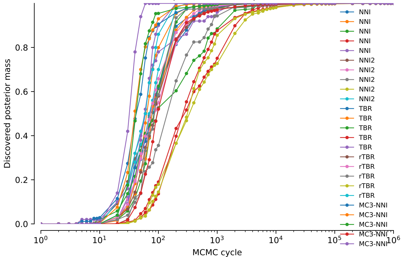
Discovered posterior mass: power = 0.02
