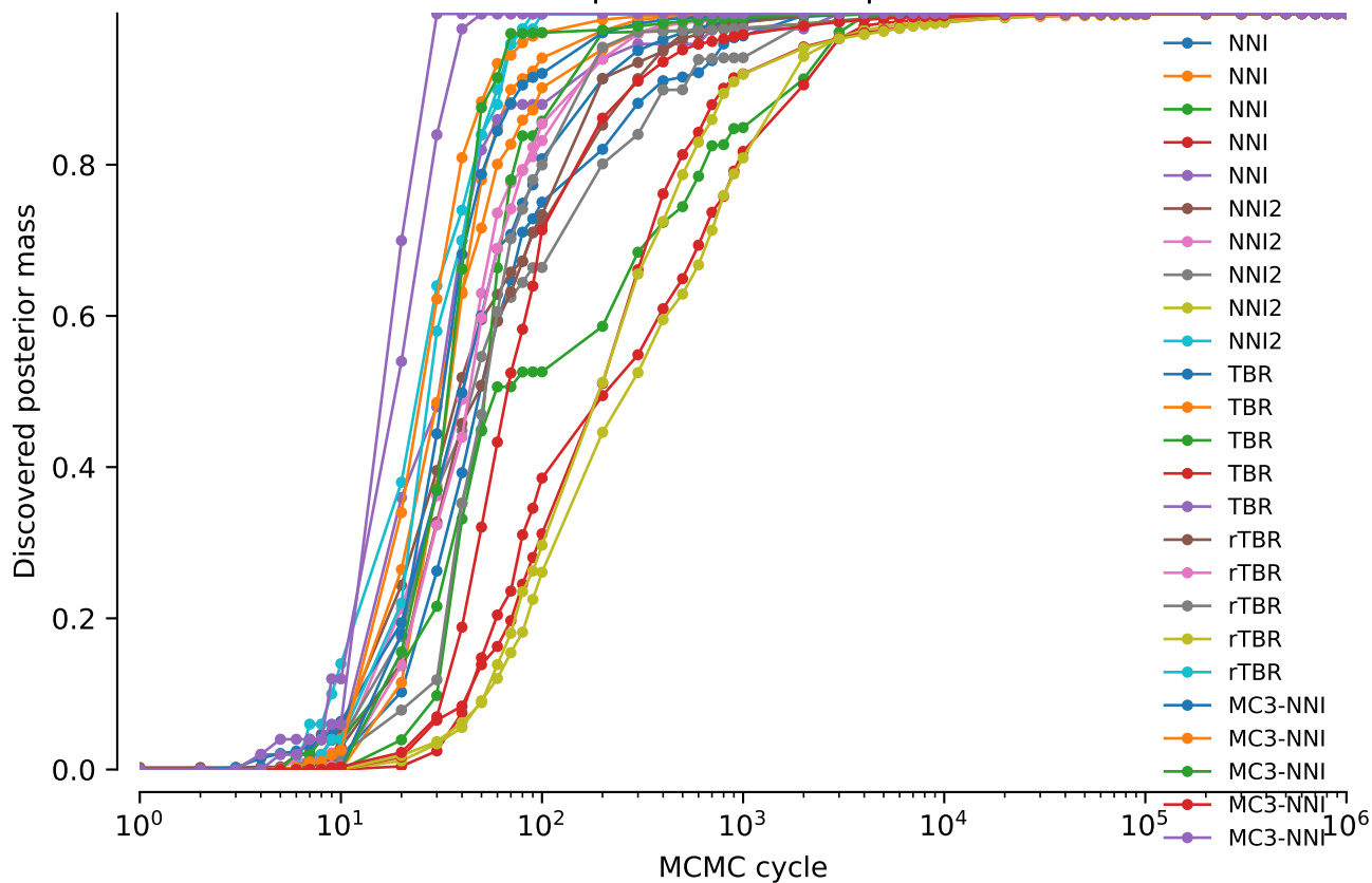
Discovered posterior mass: power = 0.05
