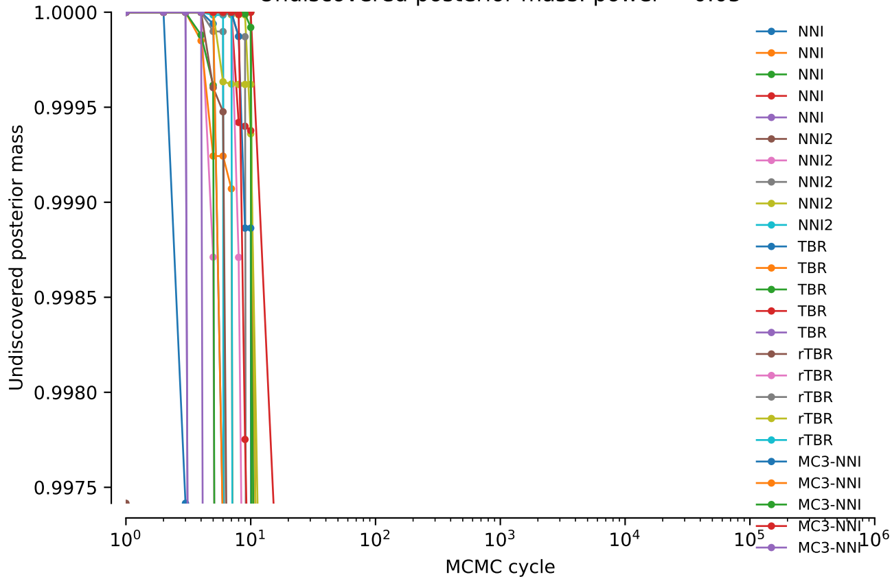
Undiscovered posterior mass: power = 0.05
