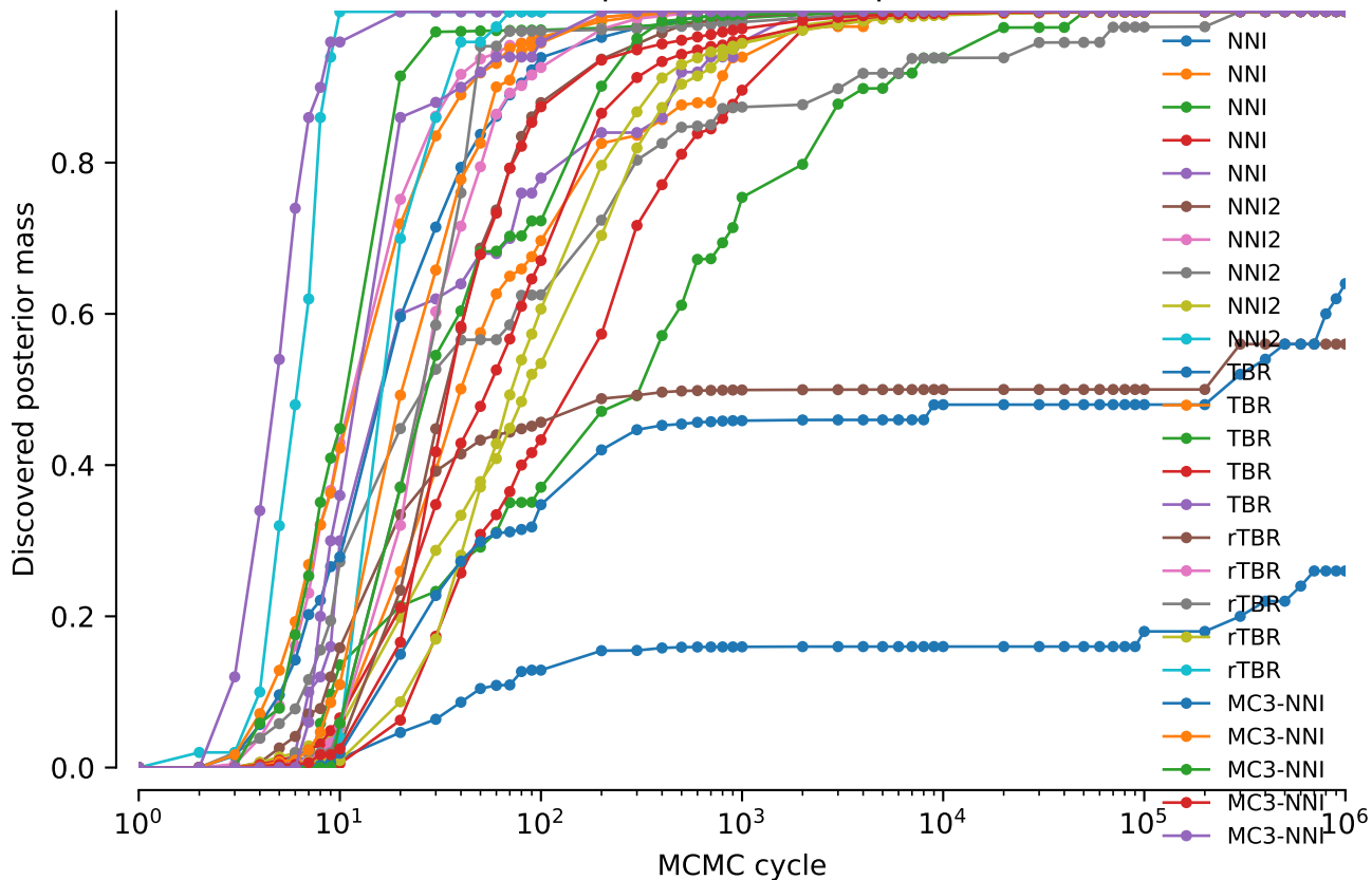
Discovered posterior mass: power = 0.2
