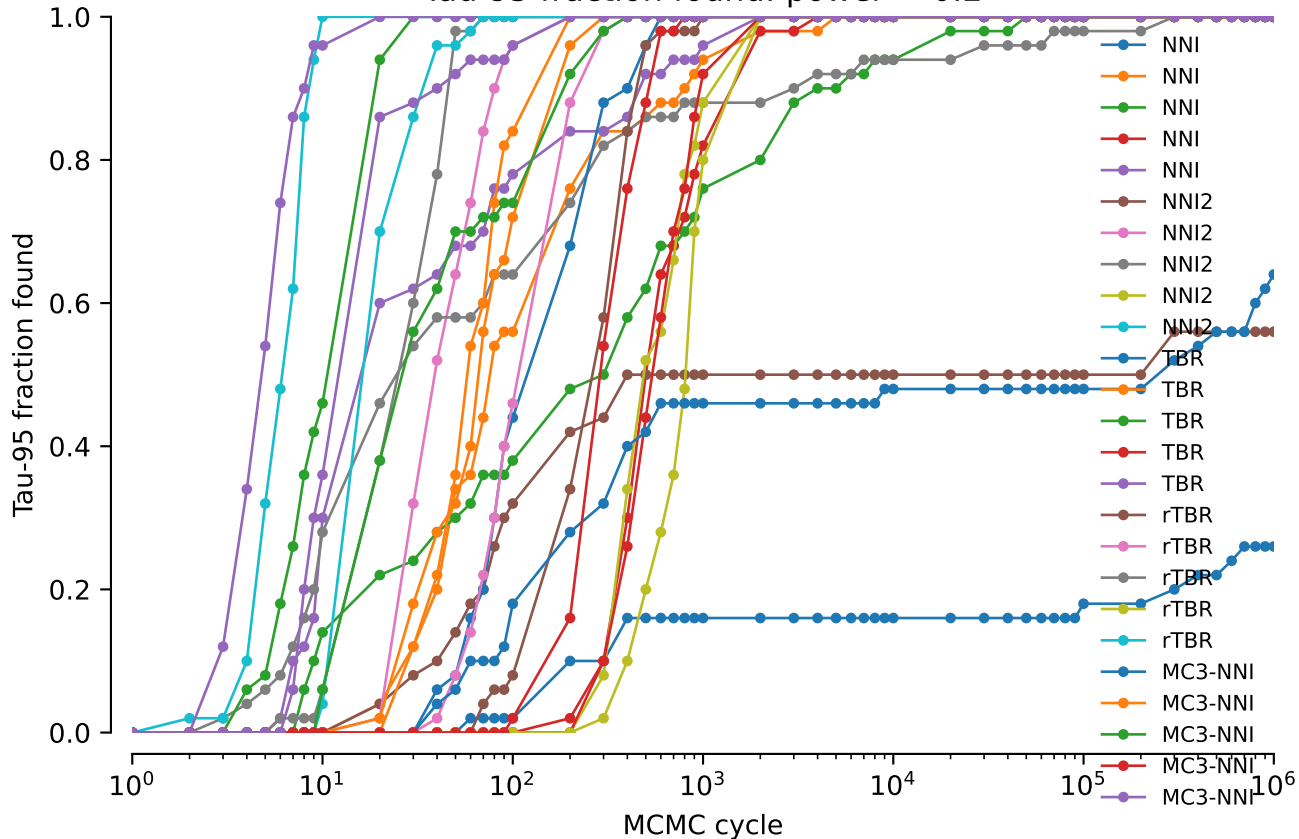
Tau-95 fraction found: power = 0.2
