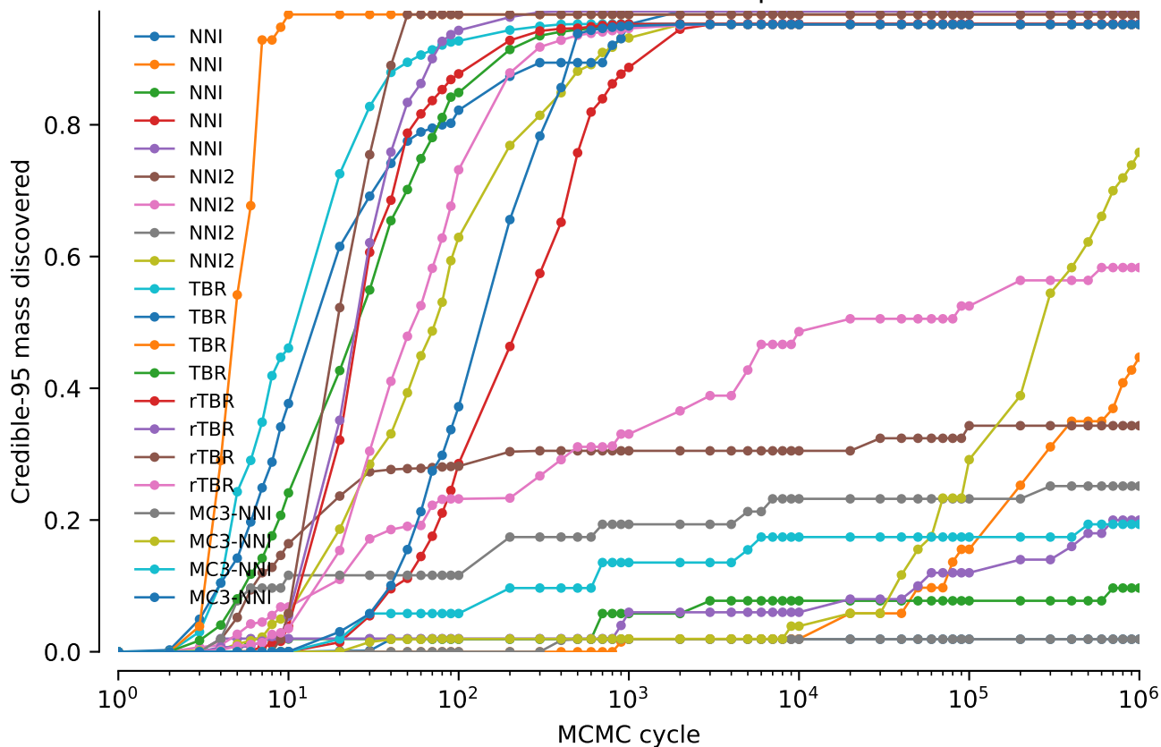
Credible-95 mass discovered: power = 0.5
