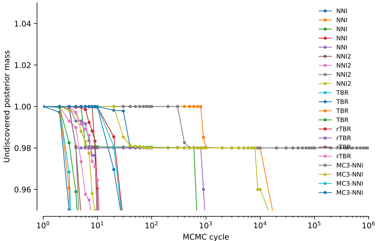
Undiscovered posterior mass: power = 0.5
