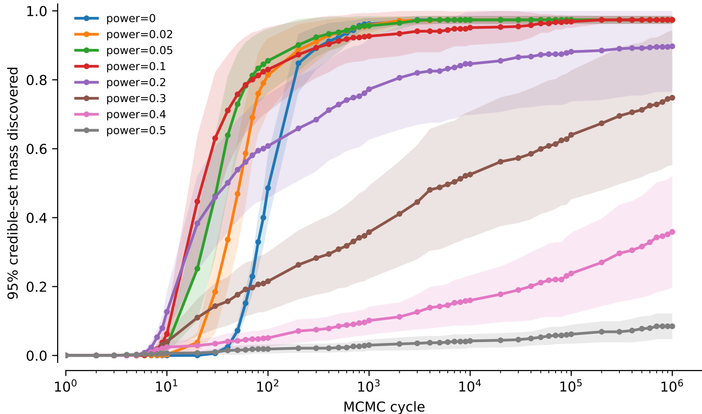
tw0: NNI powers averaged over alignments: 95% credible-set mass discovered
