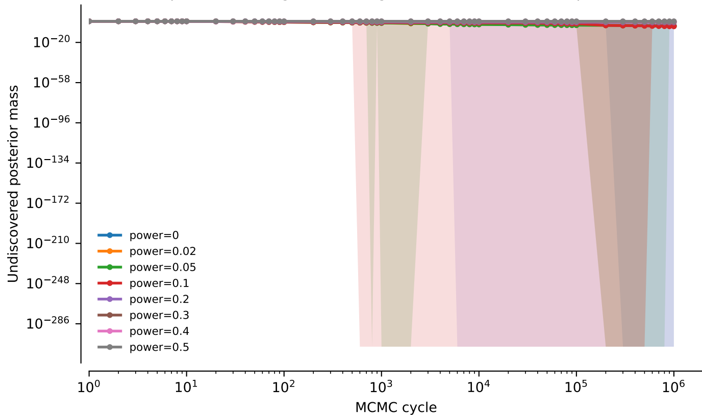
tw0: NNI powers averaged over alignments: Undiscovered posterior mass
