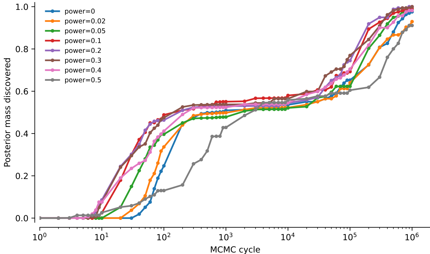
tw2: NNI powers averaged over alignments: Posterior mass discovered
