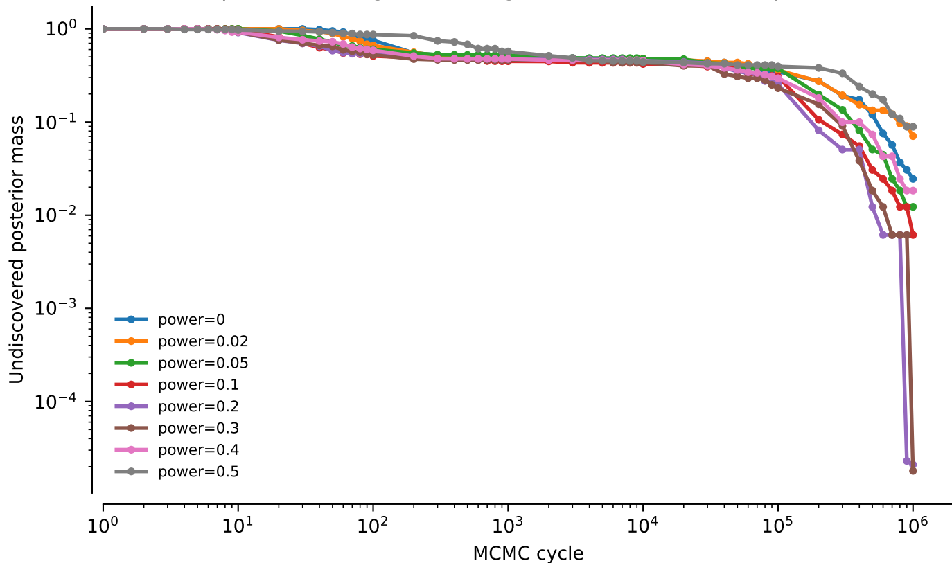
tw2: NNI powers averaged over alignments: Undiscovered posterior mass
