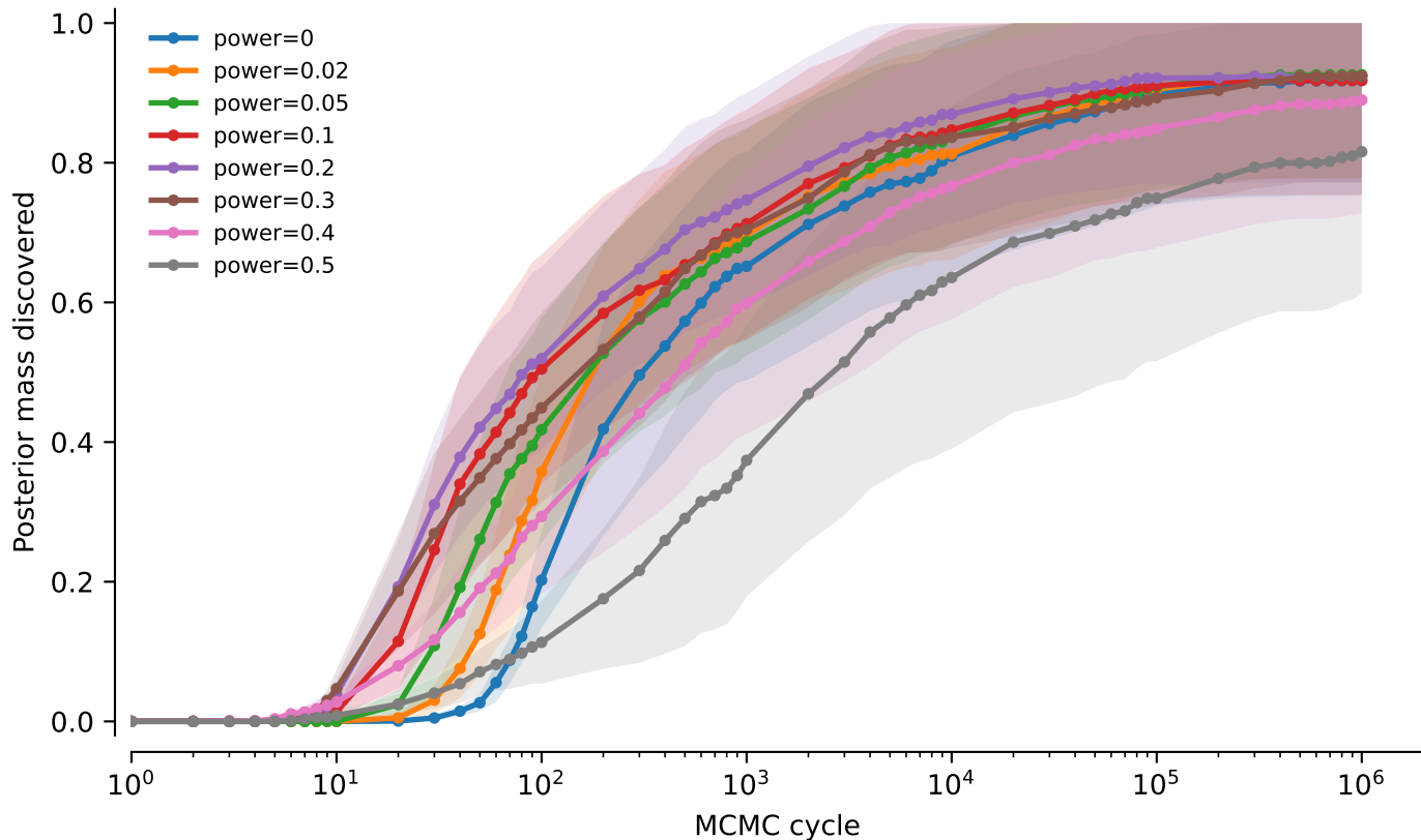
tw5: NNI powers averaged over alignments: Posterior mass discovered
