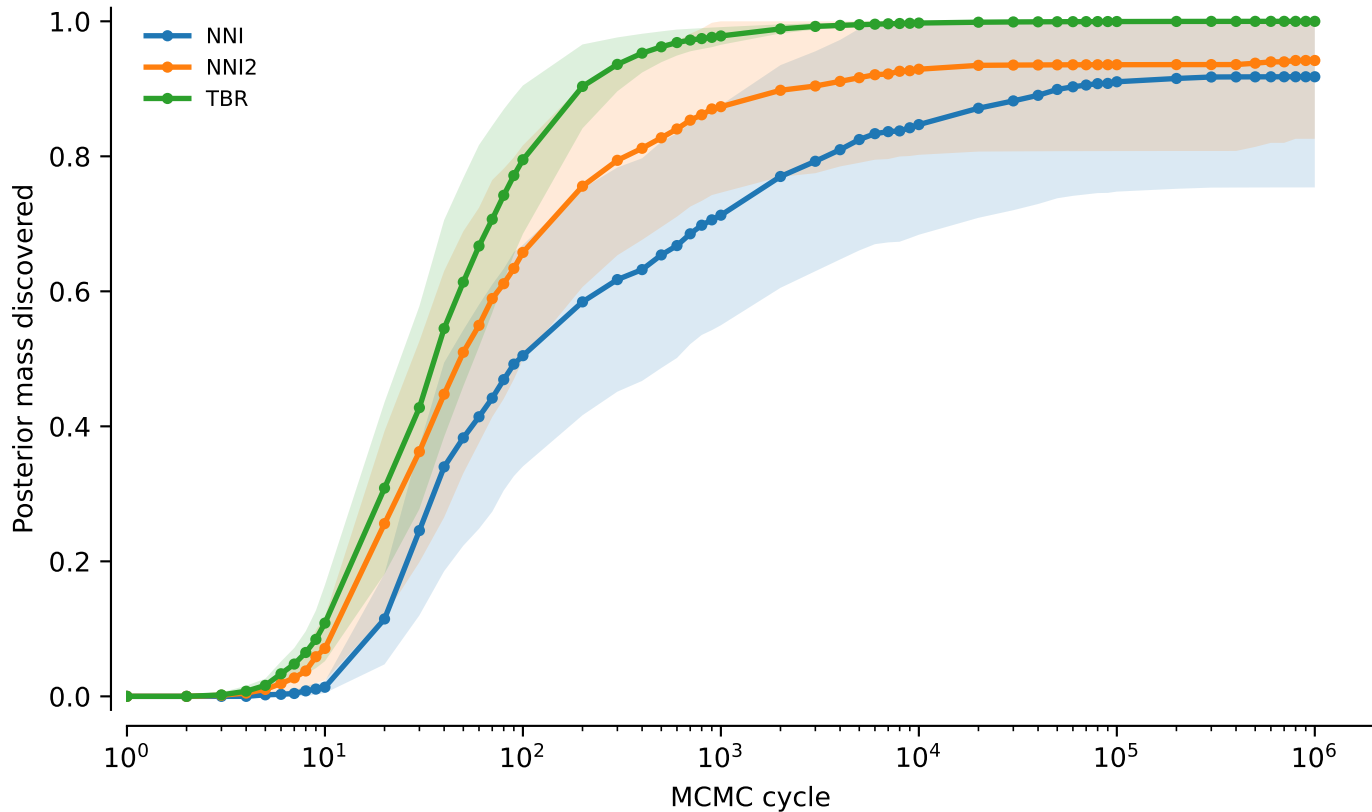
tw5: NNI vs NNI2 vs TBR, power=0.1: Posterior mass discovered
