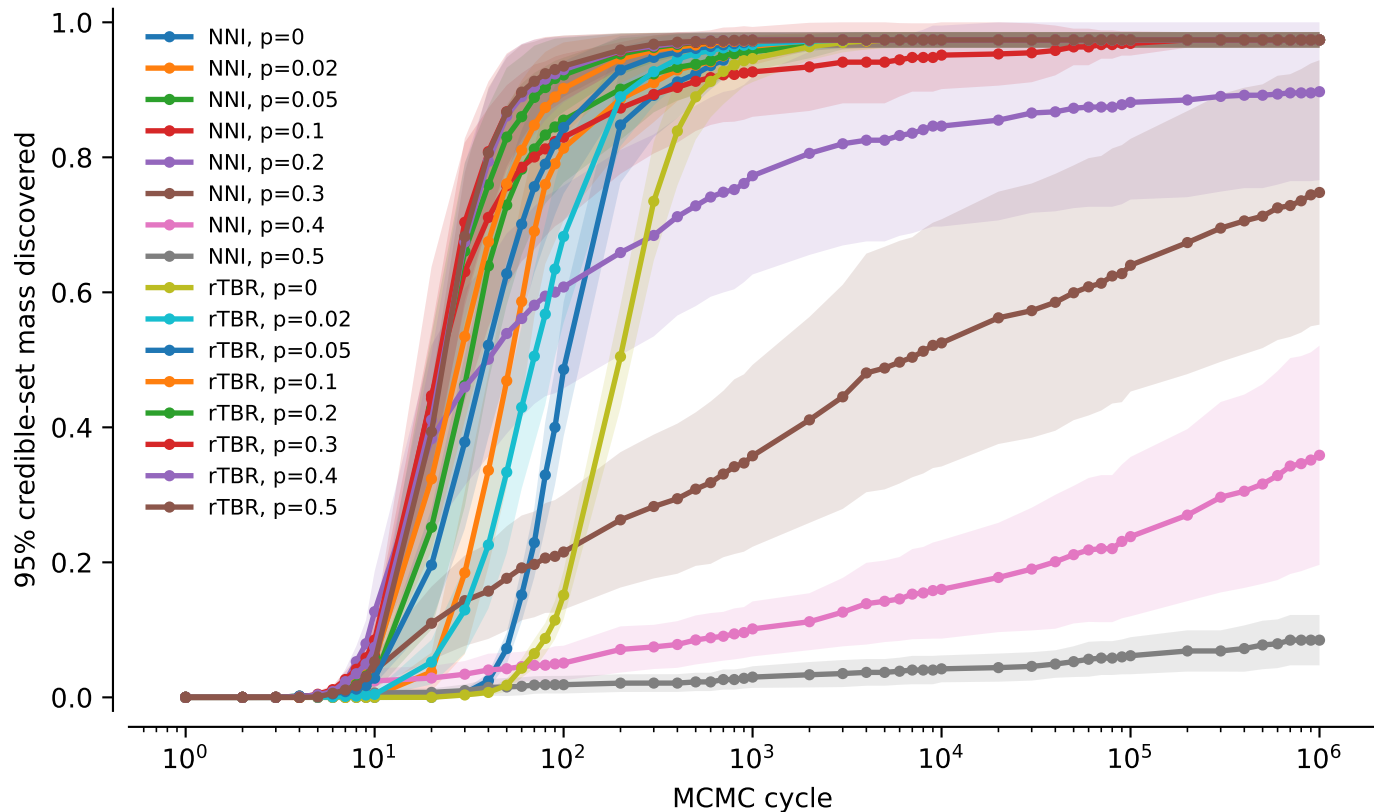
tw0: NNI vs rTBR averaged over alignments: 95% credible-set mass discovered
