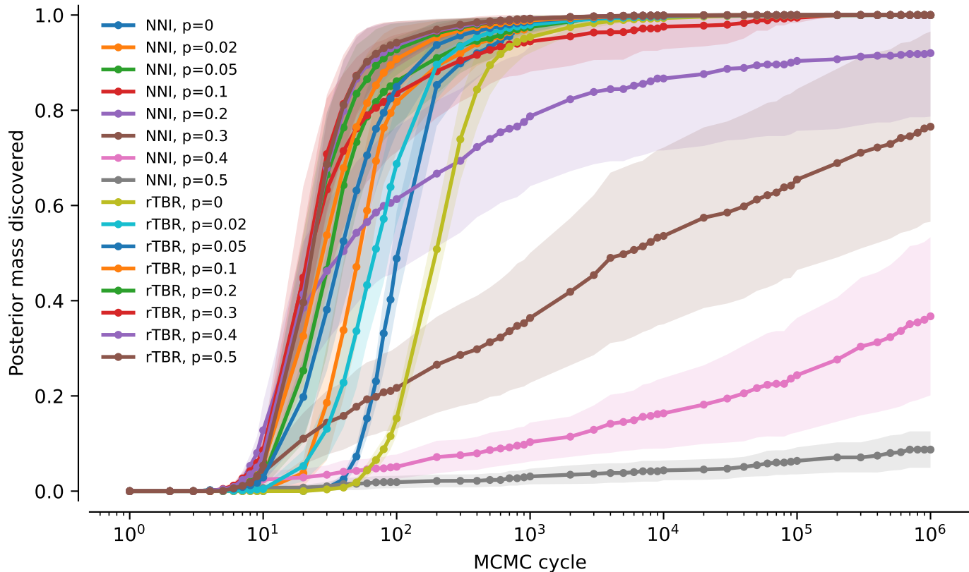
tw0: NNI vs rTBR averaged over alignments: Posterior mass discovered
