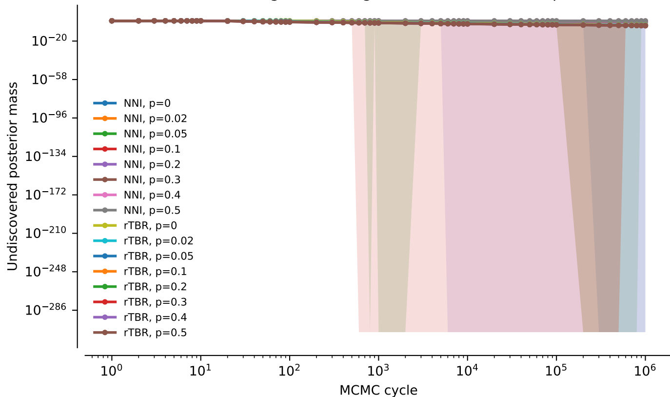
tw0: NNI vs rTBR averaged over alignments: Undiscovered posterior mass
