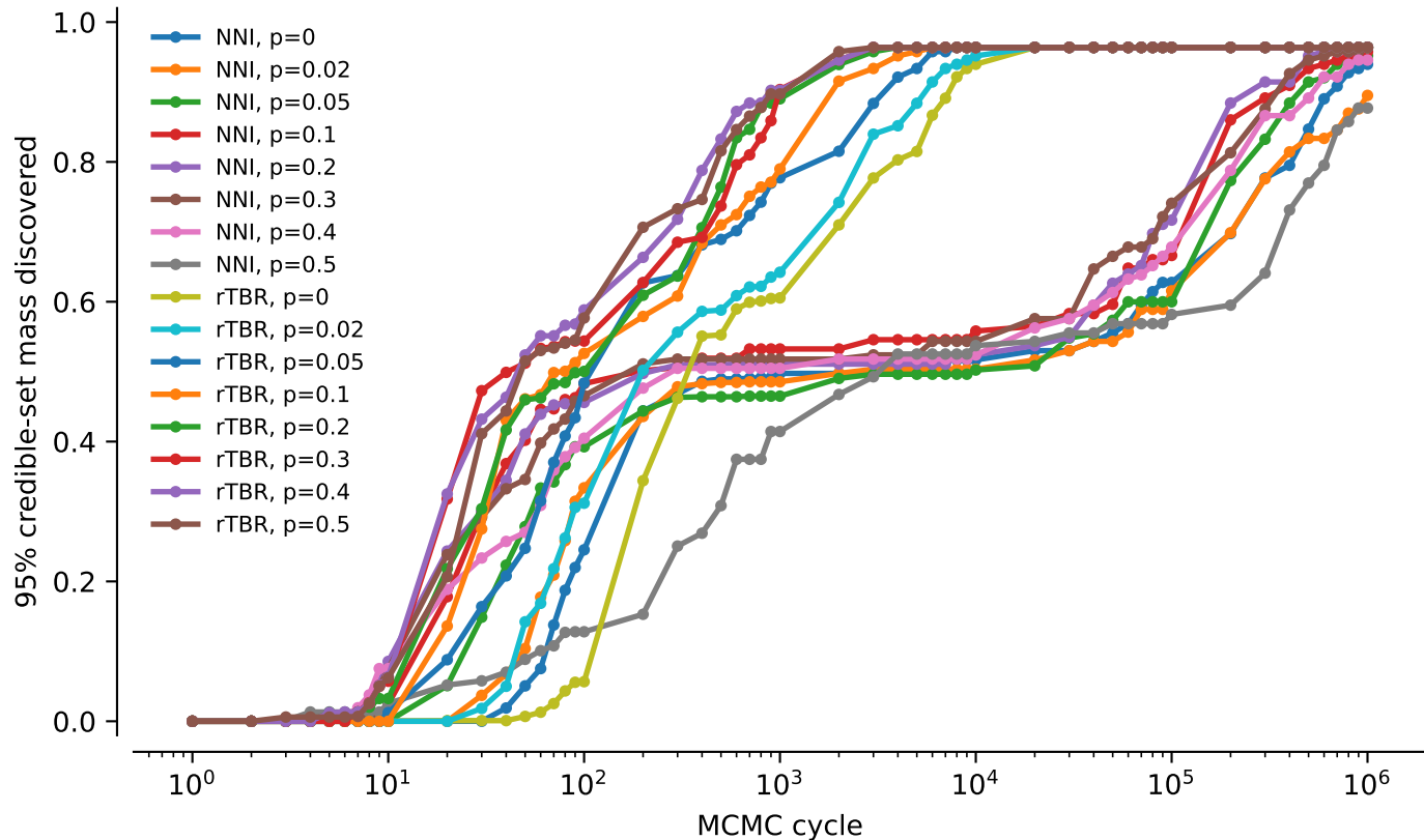
tw2: NNI vs rTBR averaged over alignments: 95% credible-set mass discovered
