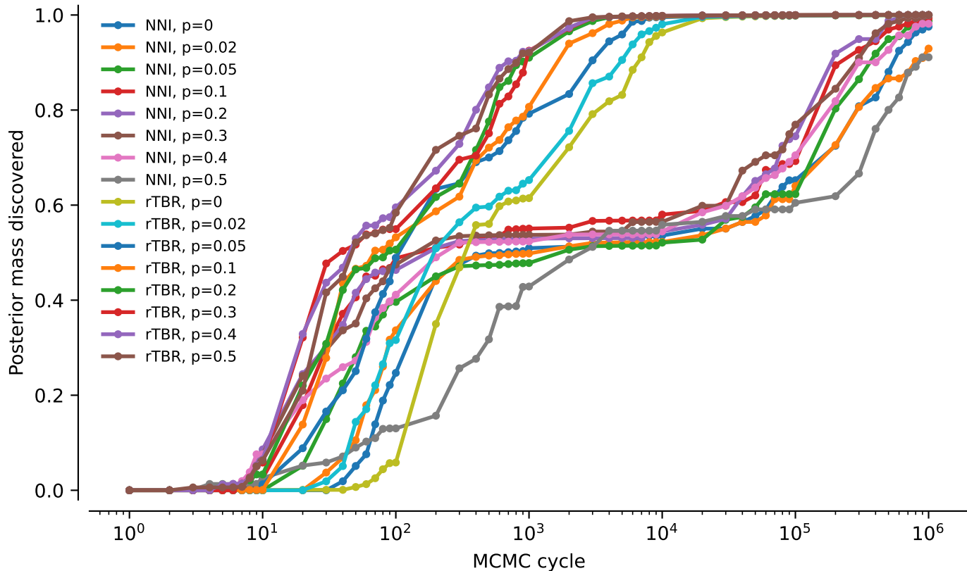
tw2: NNI vs rTBR averaged over alignments: Posterior mass discovered
