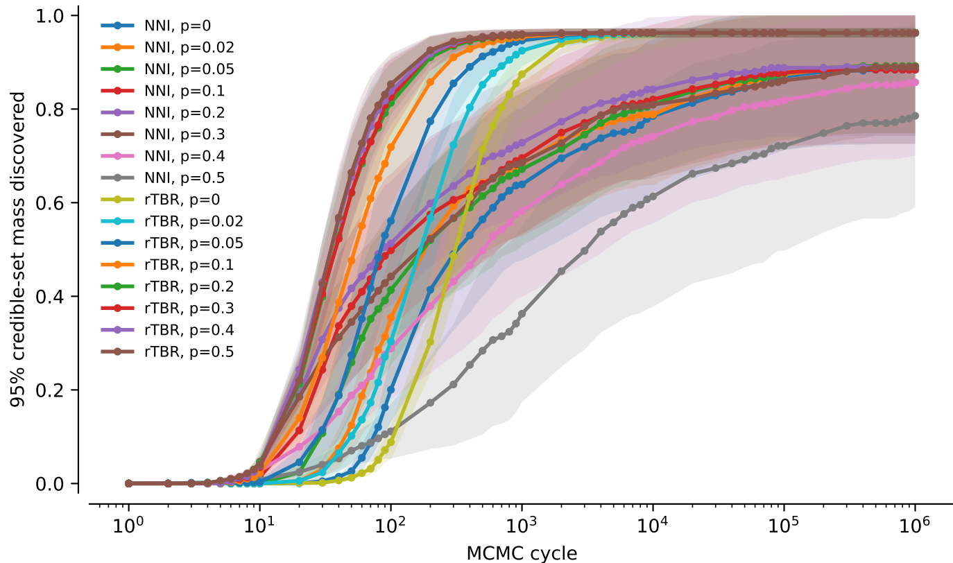
tw5: NNI vs rTBR averaged over alignments: 95% credible-set mass discovered
